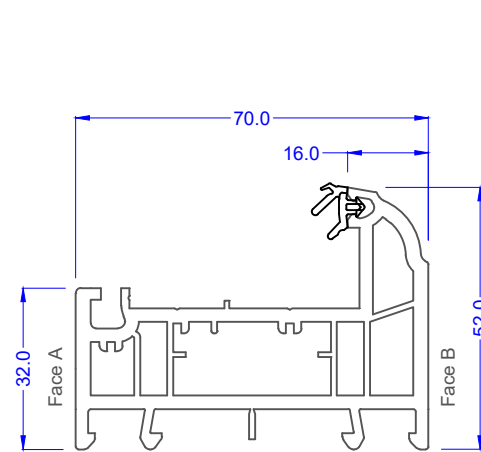
52mm Outer Frame 70S 546415 White 586415 Foiled
