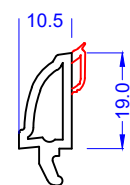
36mm Ovlo Bead 503720 White 573720 Foiled
