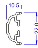
Sculptured Astragal Bar 559261 White 589261 Foiled
