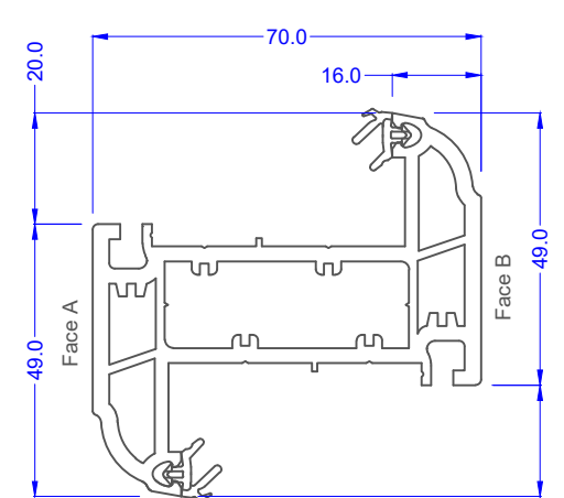
69mm Z Transom/Mullion 70S 546675 White 576675 Foiled
