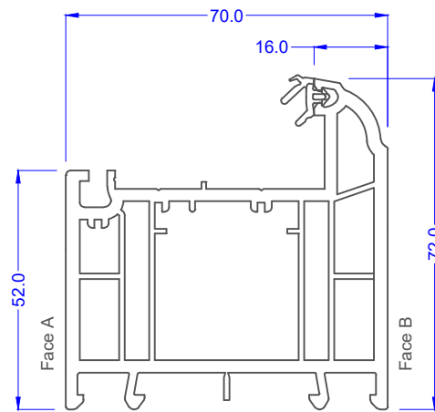
72mm Outer Frame 70S 546435 White 586435 Foiled
