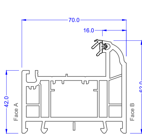
62mm Outer Frame 70S 546425 White 586425 Foiled
