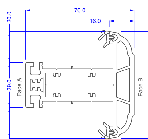
69mm T Transom/Mullion 70S 546665 White 576665 Foiled
