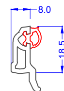
44mm Ovlo Bead 546860 White 586865 Foiled
