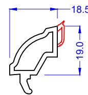
28mm Ovlo Bead 546572 White 576572 Foiled
