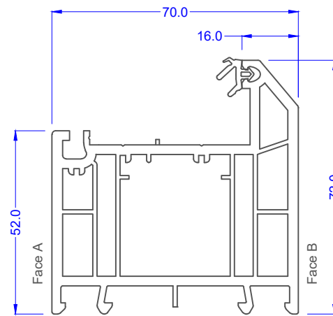
72mm Outer Frame 70C 546835 White 586835 Foiled
