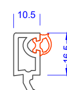
28mm Flush Sash Square Bead 559605 White 589605 Foiled
