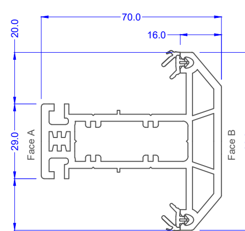
69mm T Transom/Mullion 70C 546085 White 576265 Foiled
