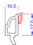
28mm Flush Sash Ovlo Bead 559600 White 589600 Foiled
