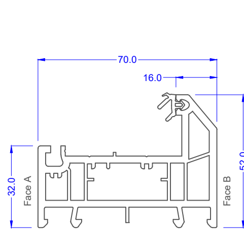
52mm Outer Frame 70C 546815 White 586815 Foiled
