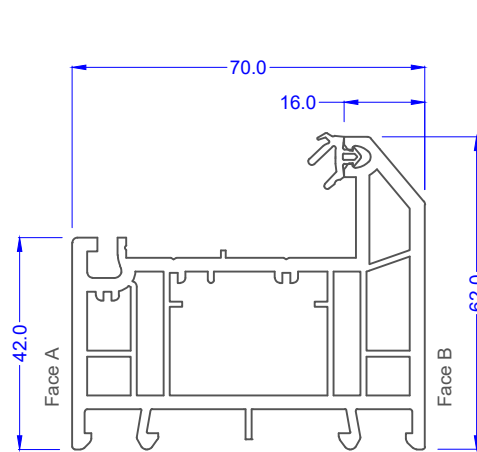
62mm Outer Frame 70C 546825 White 586825 Foiled
