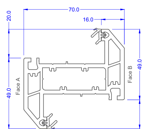
69mm Z Transom/Mullion 70C 546095 White 576275 Foiled
