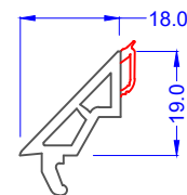
28mm Flat Bead 546132 White 576132 Foiled
