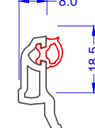
44mm Ovlo Bead 546860 White 586865 Foiled
