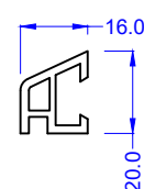
Weather Bar 561510 White
