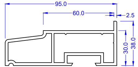
95mm Cill 546360 White 576870 Foiled
