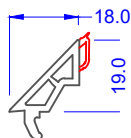
28mm Flat Bead 546132 White 576132 Foiled
