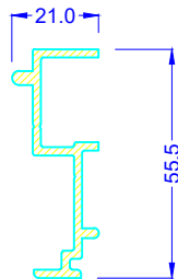
Meeting Stile Spacer 200367 Aluminium
