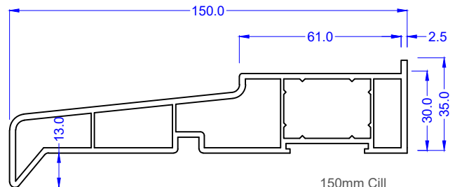
150mm Cill 246330 White 246360 Foiled
