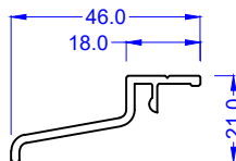
Head Drip Rail 546560 White 576231 Foiled
